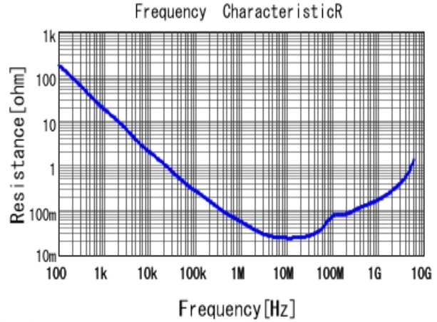
■ GRM155R61C473KA01 R DCOV, 25degC
