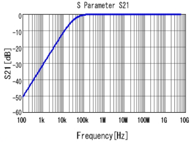
■ GRM155R61C473KA01 S21 DCOV, 25degC
