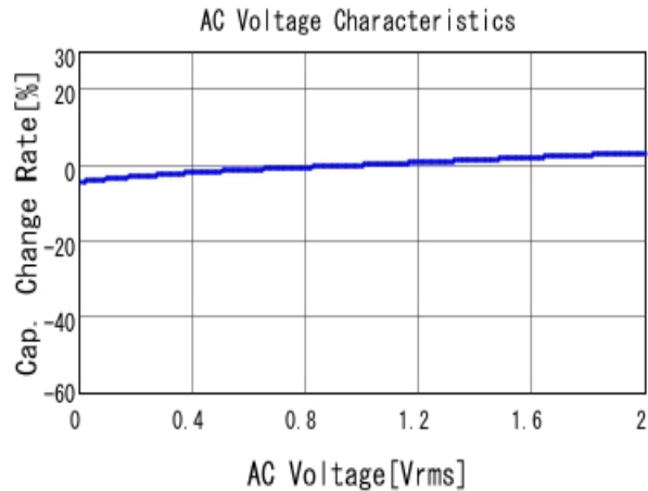
■ GRM155R61C473KA01 C-AC Voltage capchange, DCOV, 25.0d
