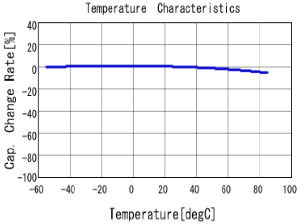
■ GRM155R61C473KA01 C-Temp. capchange, DCO. 0V, AC1.0Vrm
