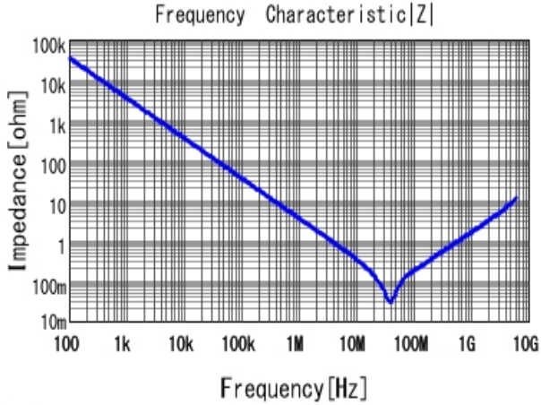
■ GRM155R61C473KA01 |Z| DCOV, 25degC
