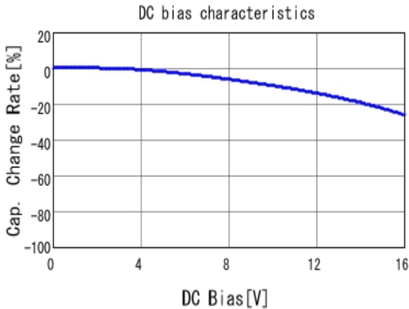
■ GRM155R61C473KA01 C-DC bias capchange, 25.0degC, AC1.
