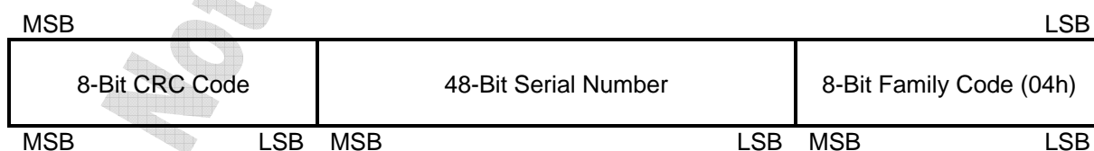
Figure 2. 64-BIT LASERED ROM
