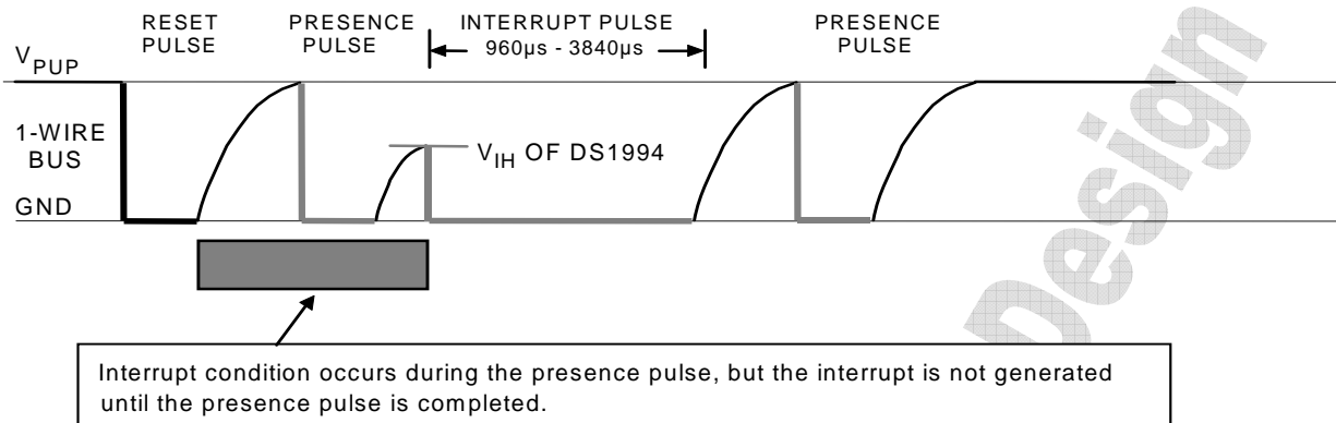
Figure 14. TYPE 2 INTERRUPT
