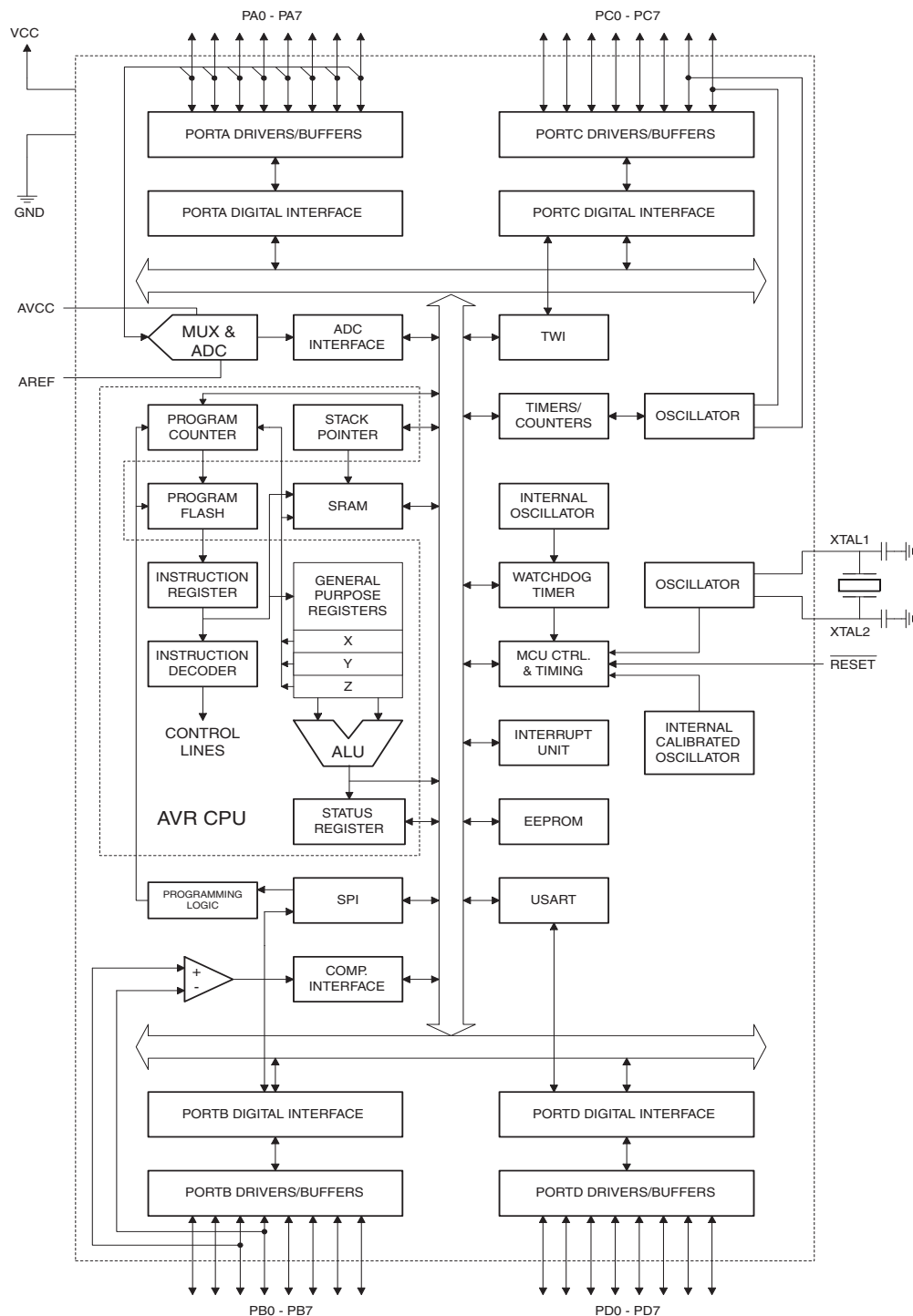
Figure 2-1. Block Diagram
