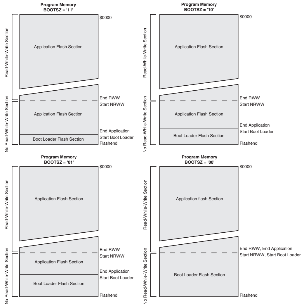
Figure 25-2. Memory Sections (1)
