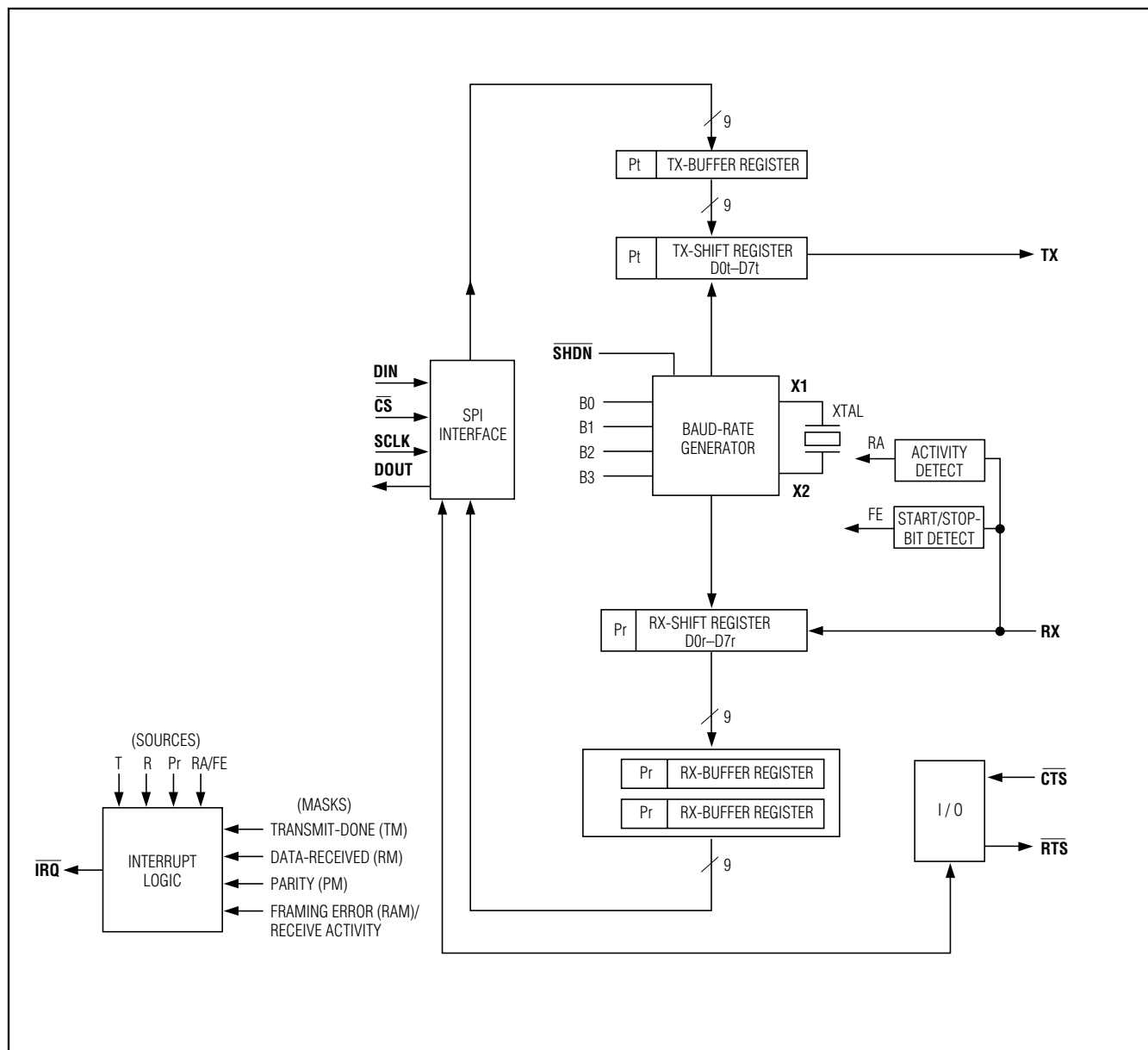
Figure 2. Functional Diagram
