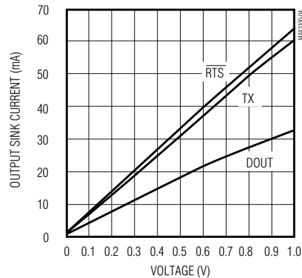
TX, \overline{\text{RTS}} , DOUT OUTPUT CURRENT vs. OUTPUT LOW VOLTAGE ( V_{CC} = 3.3\text{V} )
