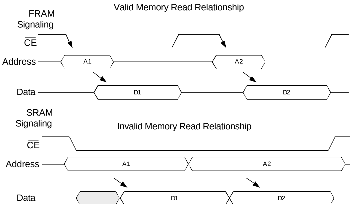
Figure 4. Memory Address Relationships
