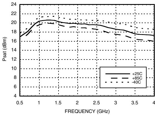
Psat vs. Temperature @ Vdd = +5V
