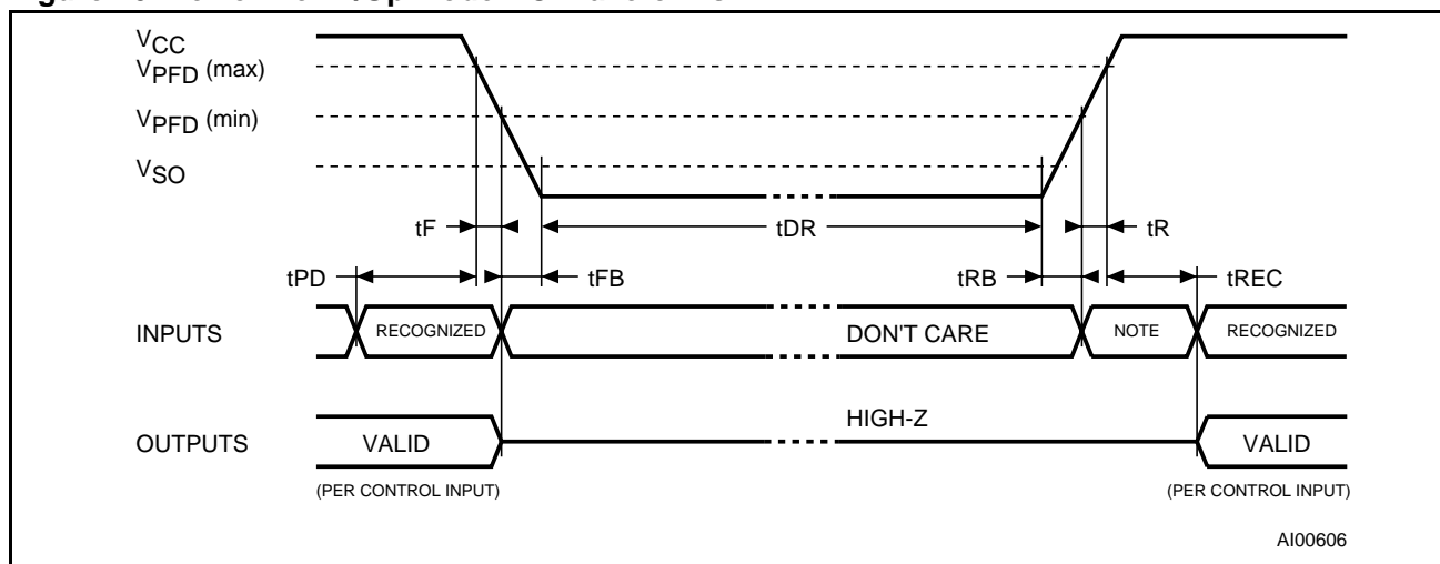
Figure 10. Power Down/Up Mode AC Waveforms
