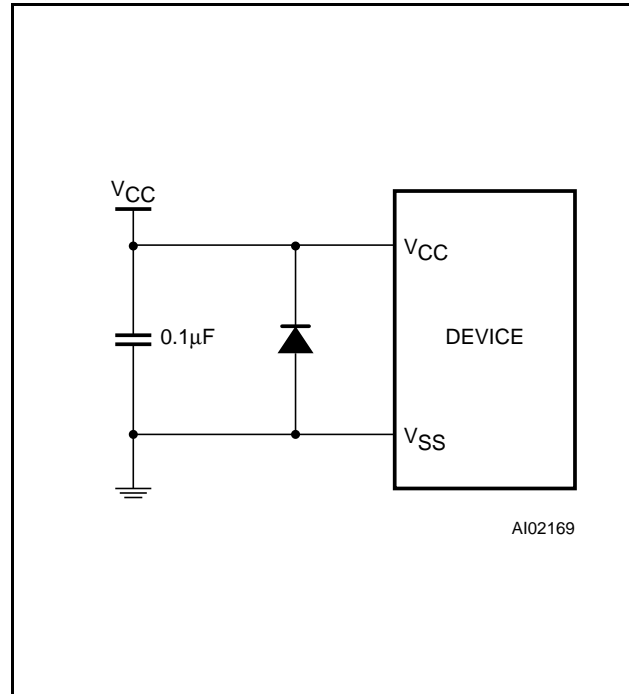
Figure 12. Supply Voltage Protection
