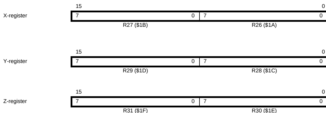
Figure 7. X, Y and Z-registers
