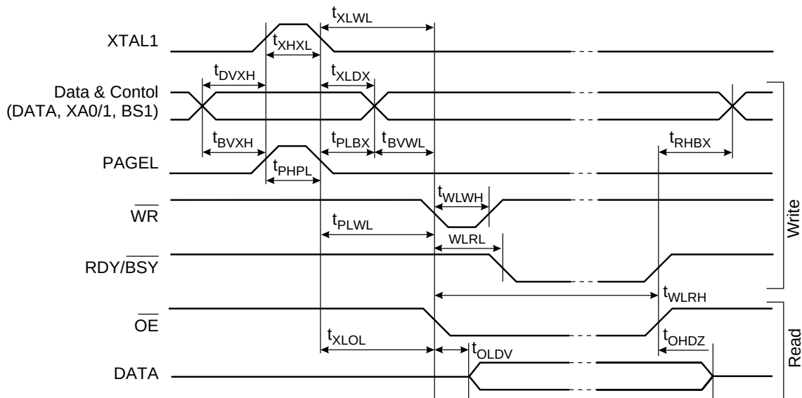
Figure 80. Parallel Programming Timing
