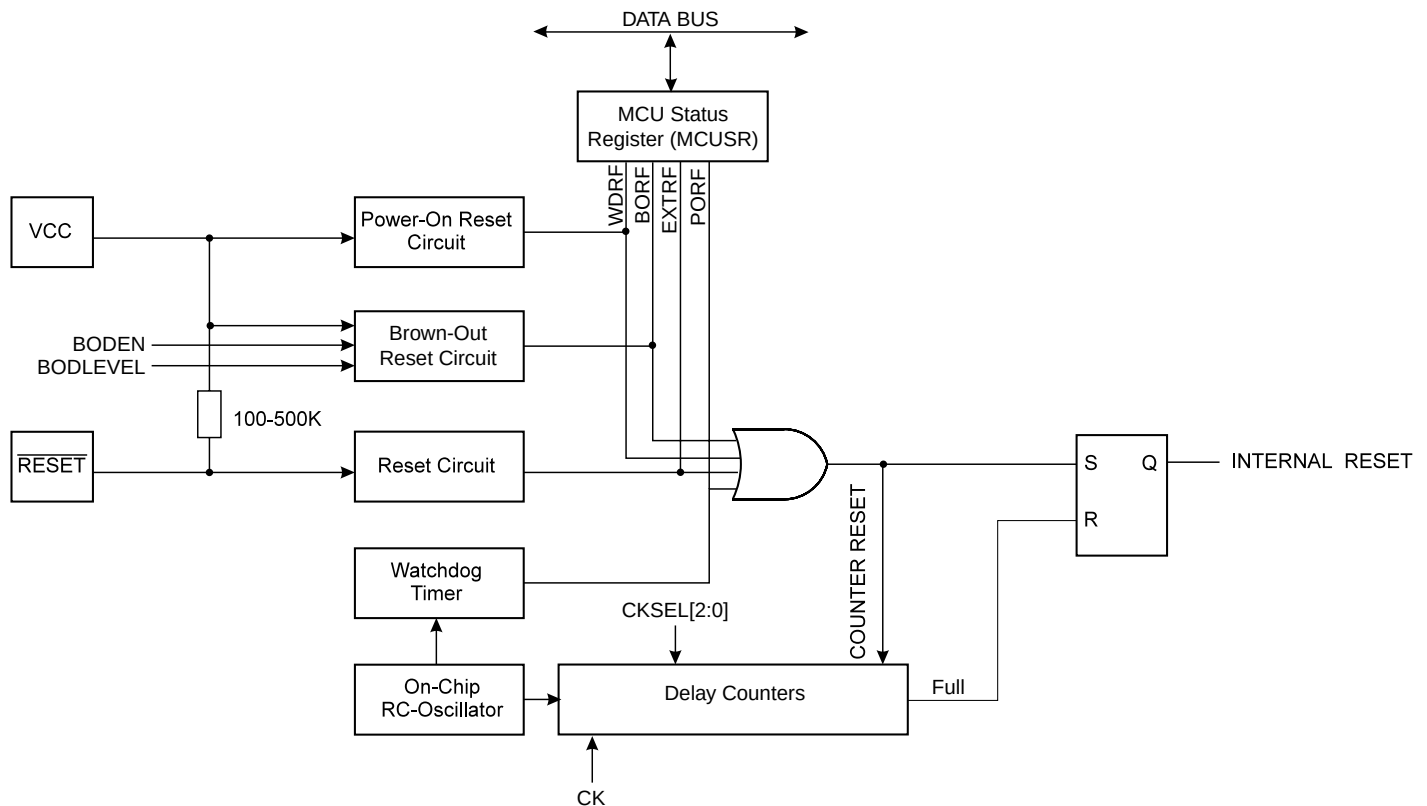
Figure 24. Reset Logic
