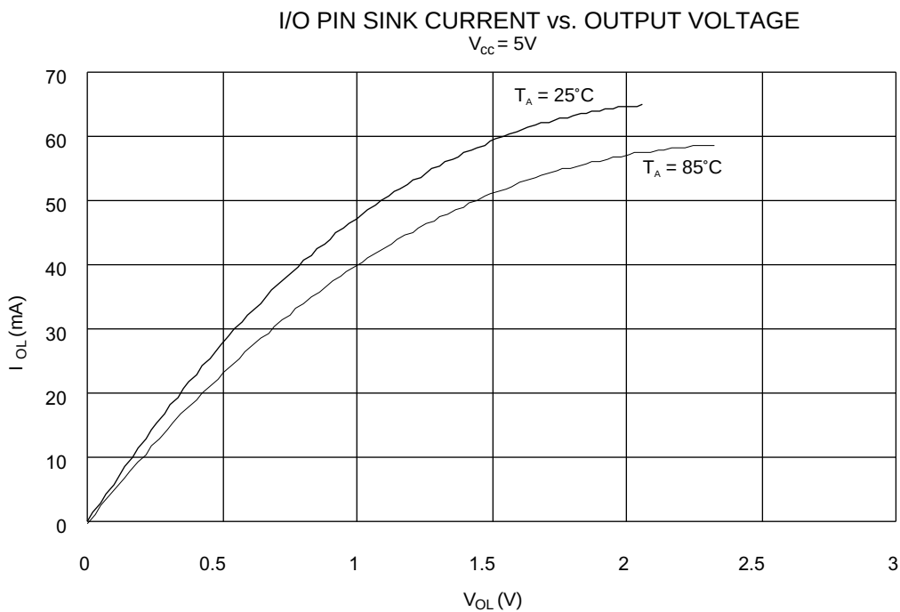
Figure 94. I/O Pin Sink Current vs. Output Voltage
