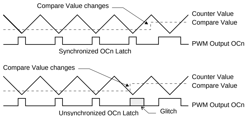
Figure 35. Effects of Unsynchronized OCR Latching in overflow mode.
