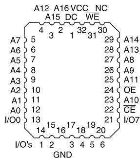
PLCC Top View
