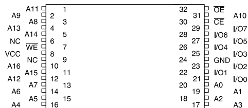
TSOP Top View
