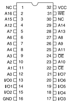
PDIP Top View
