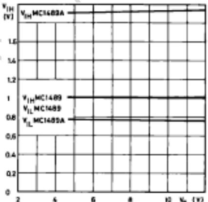
Figure 14. Input threshold vs power supply voltage
