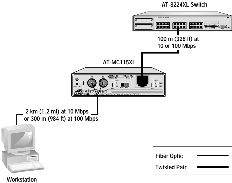
Figure 4 Standalone Topology
