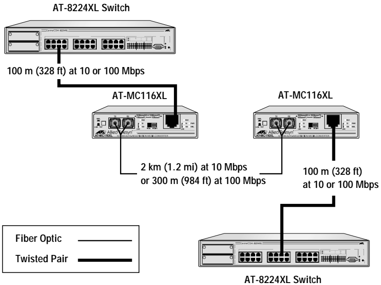
Figure 5 Back-to-Back Topology
