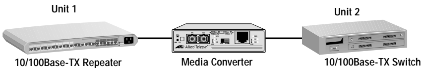
Figure 3 Example of a Duplex Mode Mismatch
