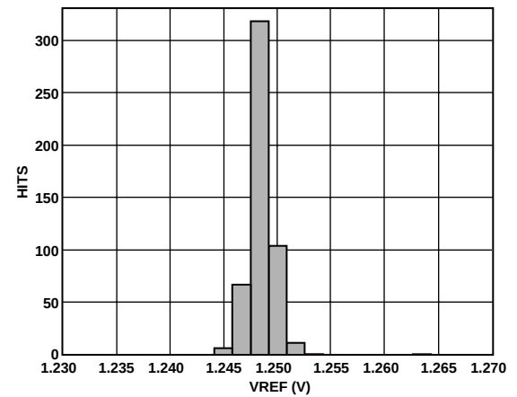
Figure 37. VREF Distribution
