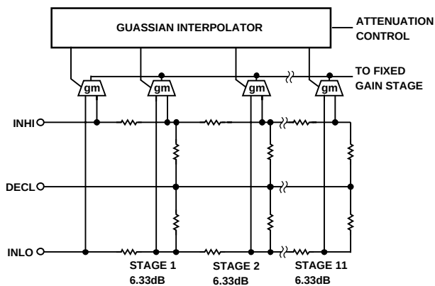
Figure 52. Simplified Input Circuit
