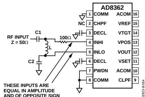
Figure 54. Narrow-Band Reactive Input Coupling
