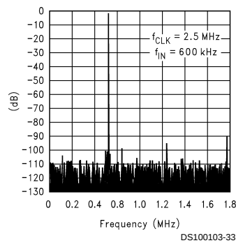
Spectral Response
