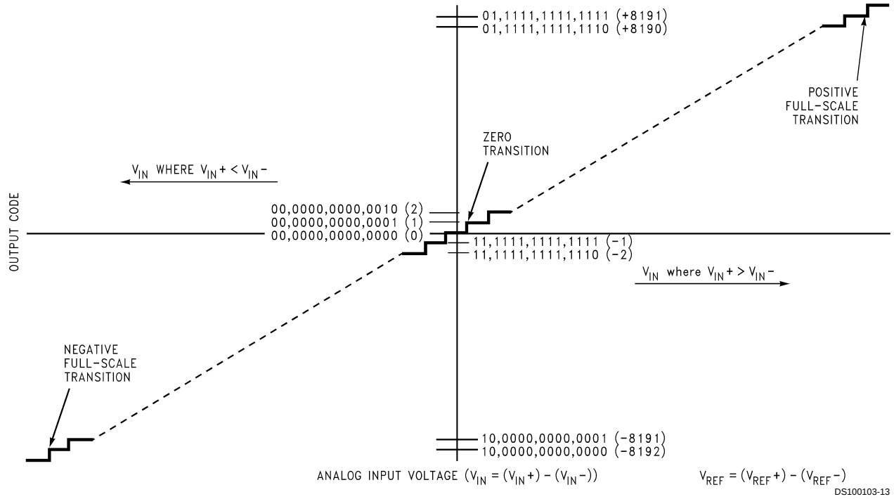
FIGURE 1. Transfer Characteristics
