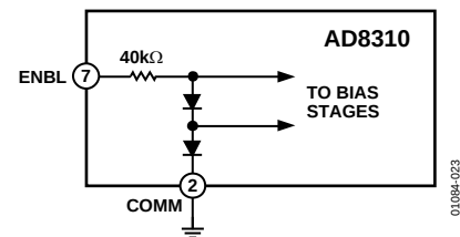
Figure 23. Enable Interface
