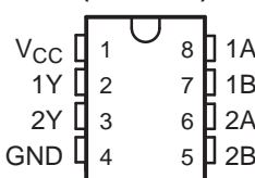
D PACKAGE (TOP VIEW)
