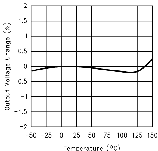
Figure 6. Temperature Stability
