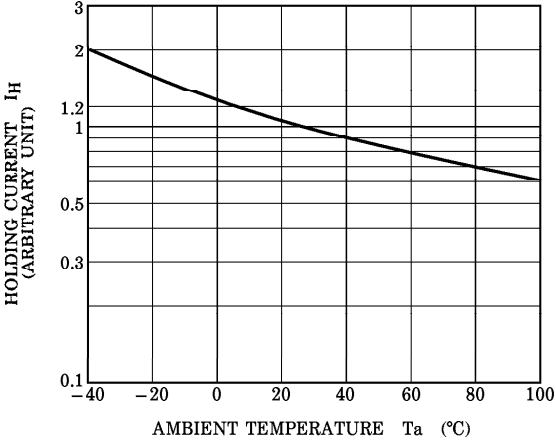
NORMALIZED I_H - T_a
