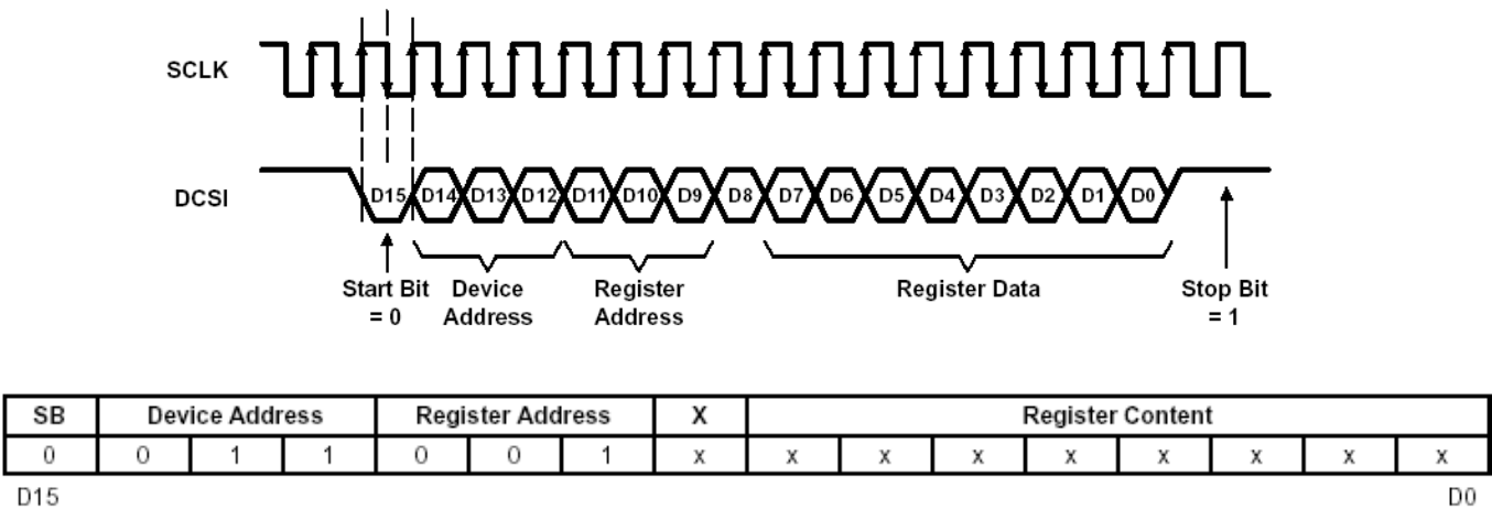
Figure 2: TLV320AIC10 configuration timing via DCSI port
