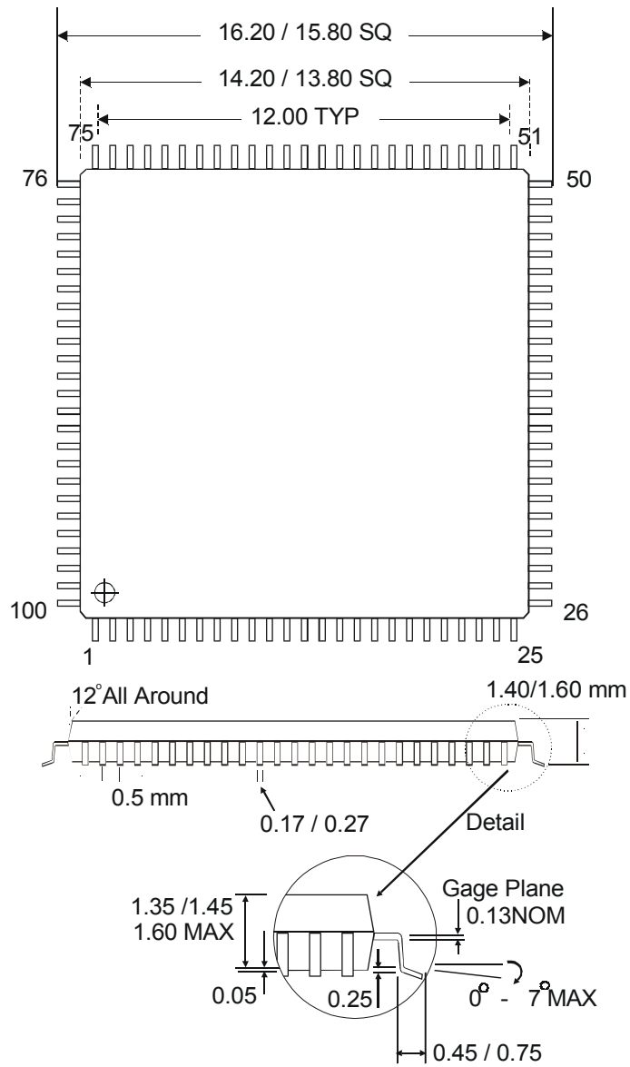
Figure 3-E Package Dimensions
