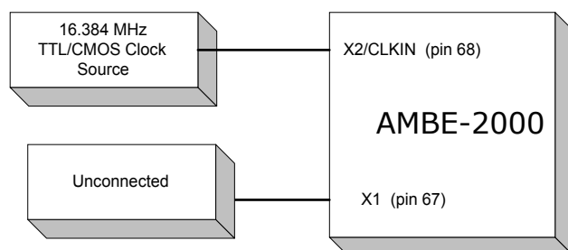
Figure 3-C X2/CLKIN and X1 with TTL Clock Source
