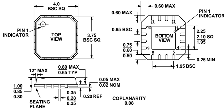
Figure 64. 16-Lead Lead Frame Chip Scale Package [LFCS] 4 mm x 4 mm Body (CP-16) Dimensions shown in millimeters
