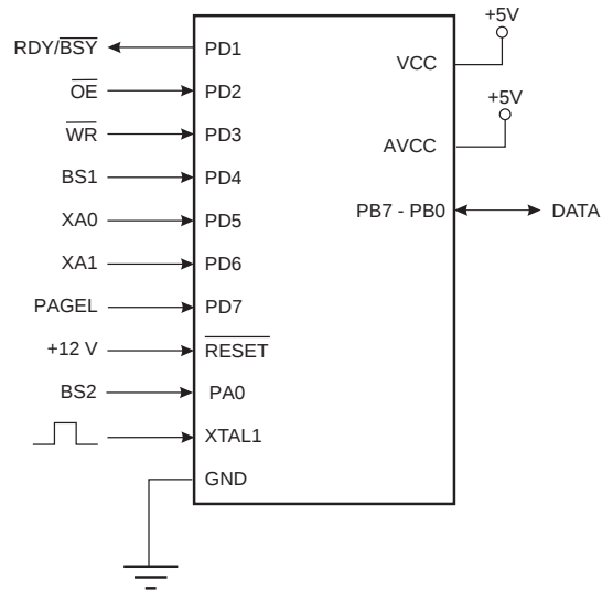
Figure 29-1. Parallel Programming (1)
