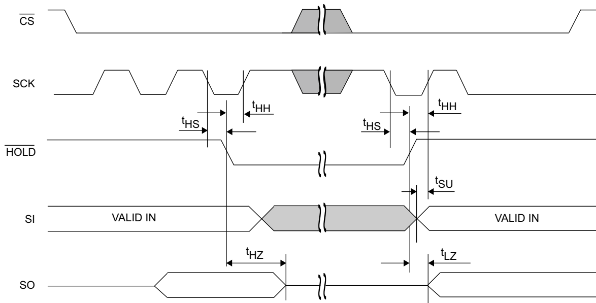
Figure 16. HOLD Timing
