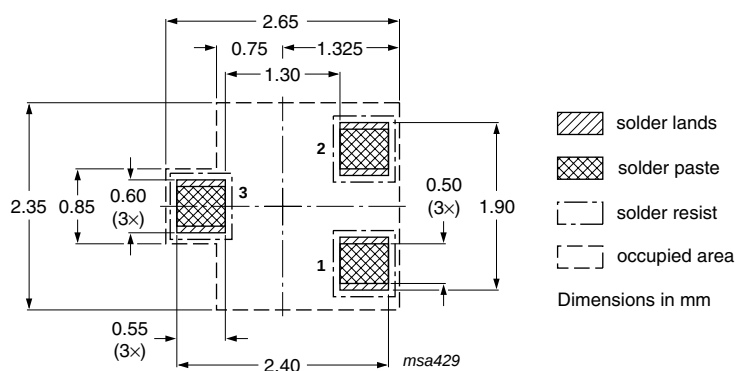
Fig 21. Reflow soldering footprint SOT323 (SC-70)
