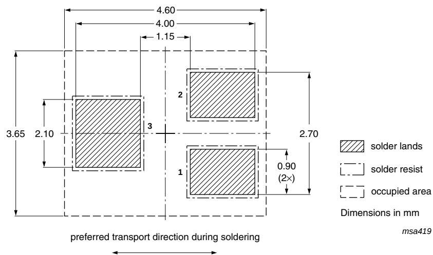
Fig 22. Wave soldering footprint SOT323 (SC-70)
