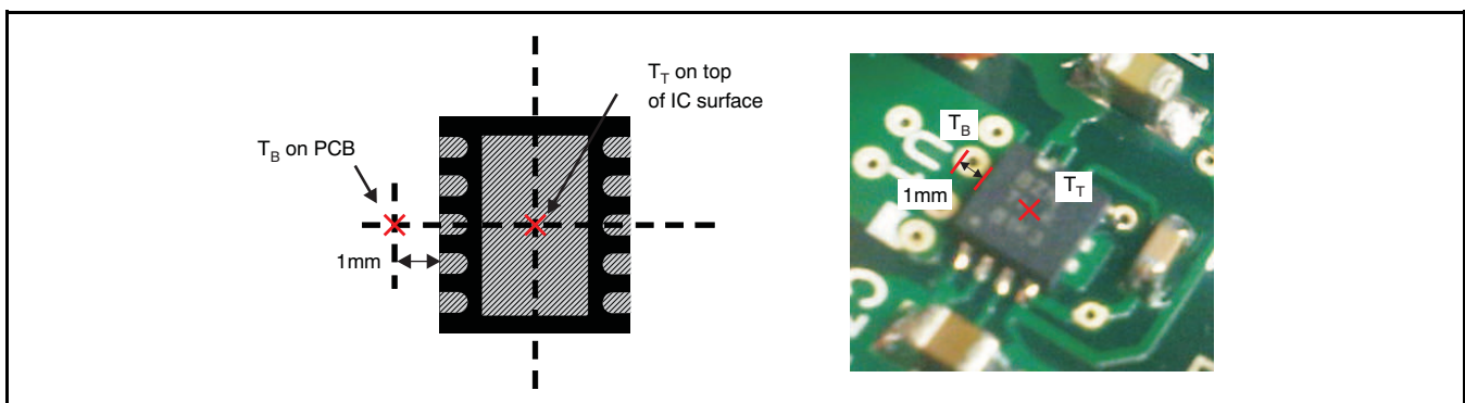
Figure 30. Measuring Points for T T and T B
