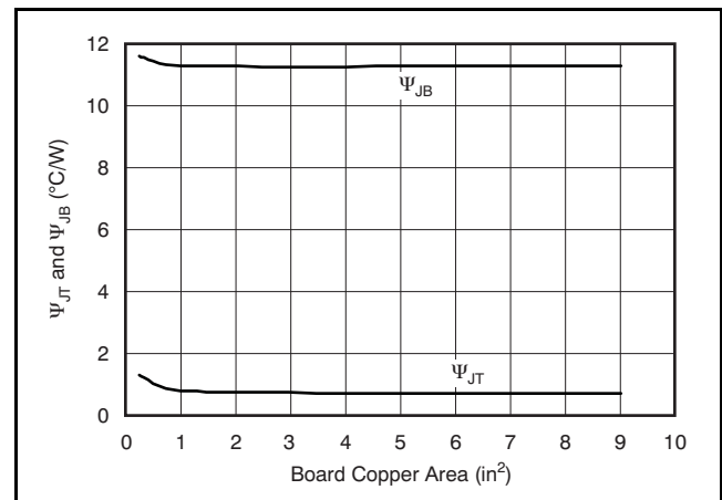
Figure 29. Ψ JT and Ψ JB vs Board Size
