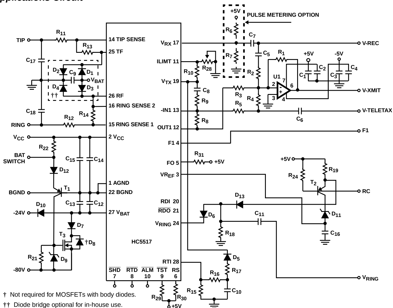
FIGURE 15. APPLICATION CIRCUIT
