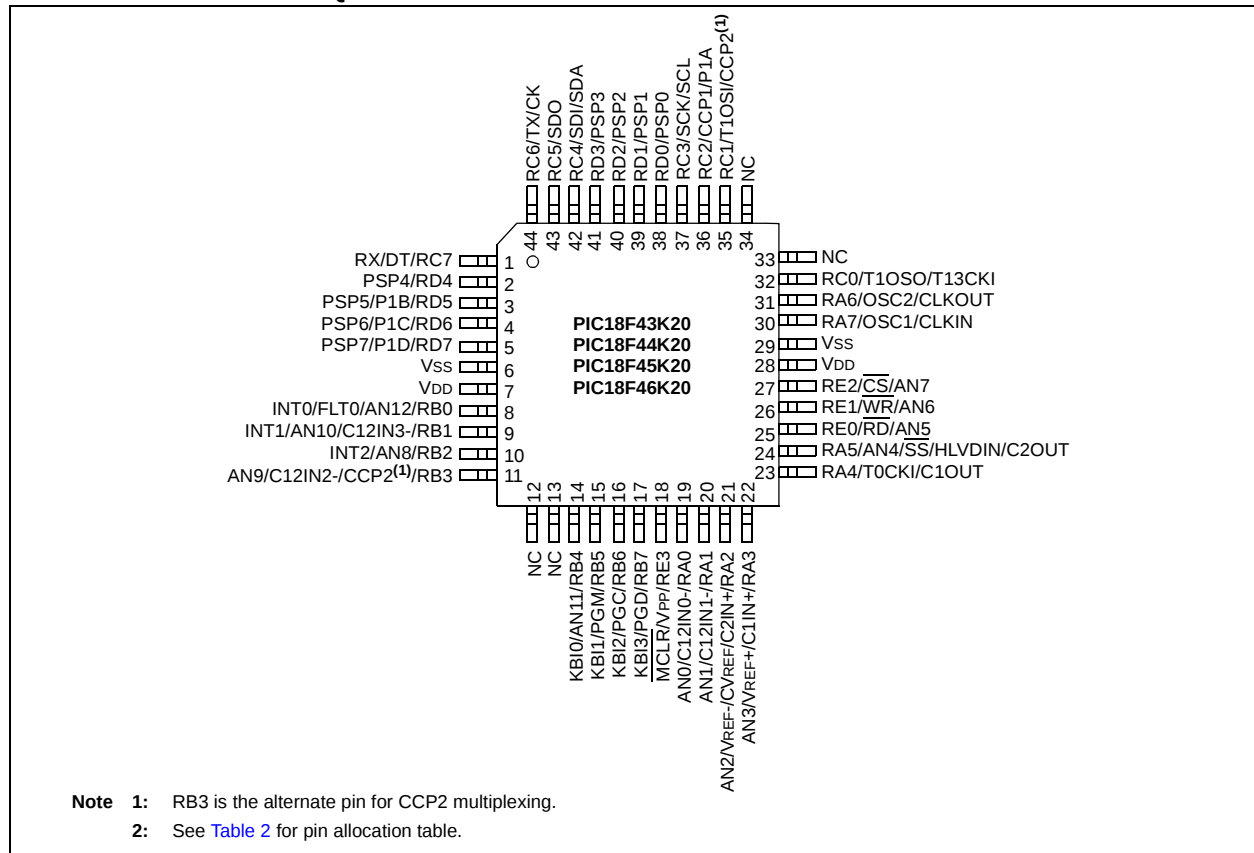
FIGURE 6: 44-PIN TQFP
