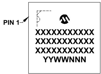
44-Lead TQFP (10x10x1 mm)
