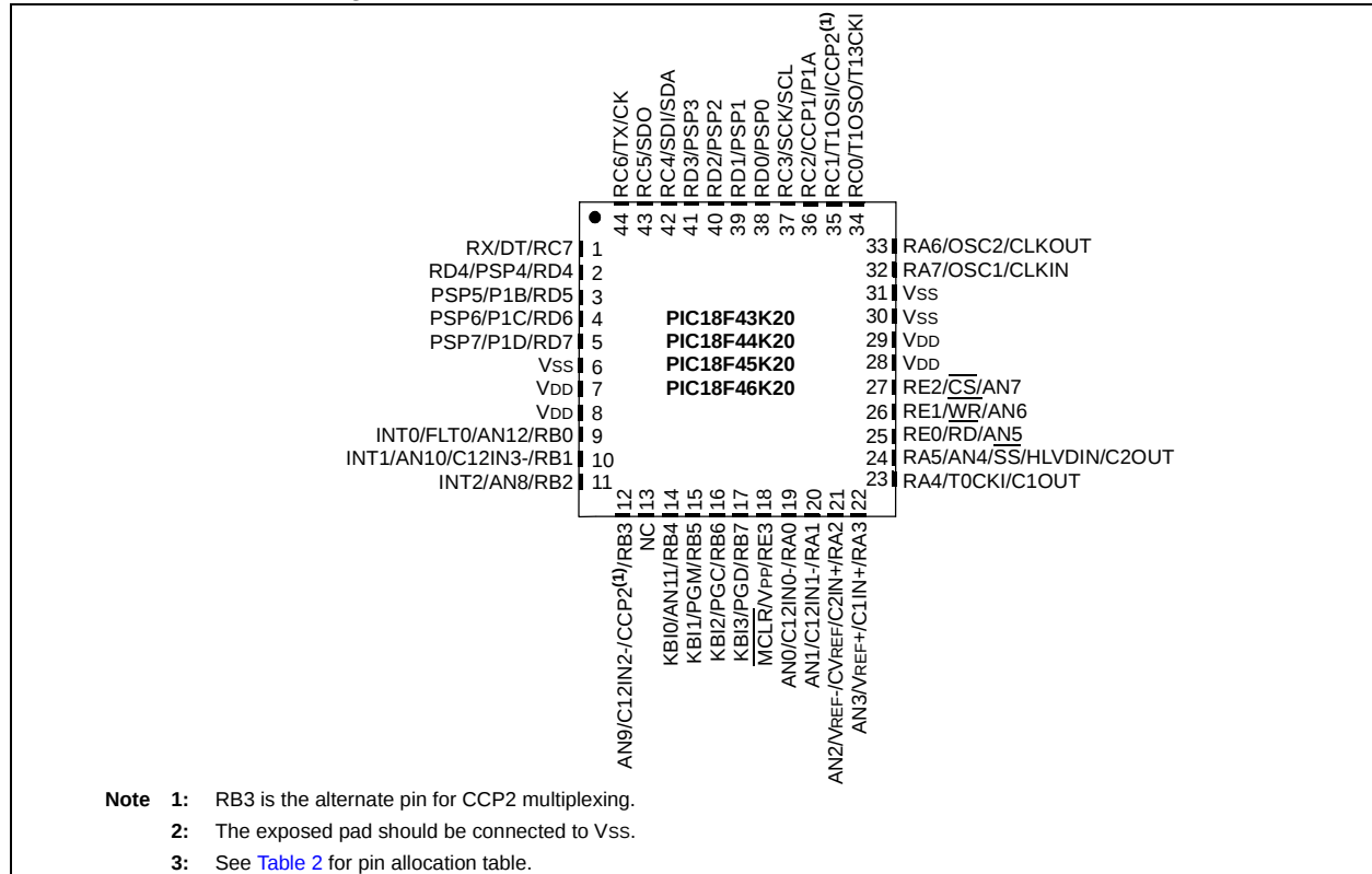
FIGURE 5: 44-PIN QFN
