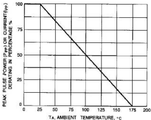
Fig. 2-PULSE DERATING CURVE
