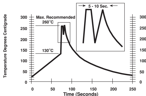
Recommended Solder Profile — Wave Solder
