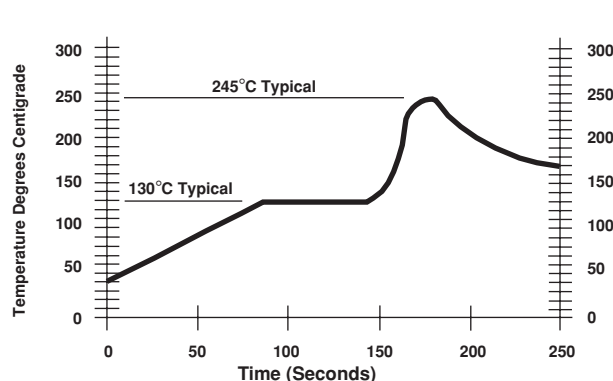
Recommended Solder Profile — Reflow
