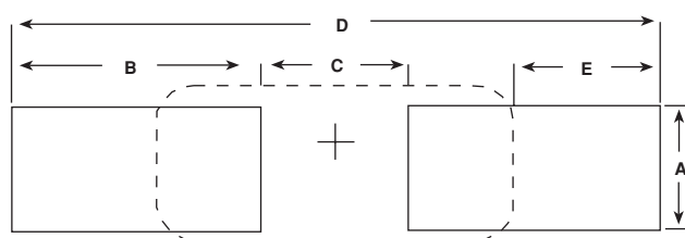
Wave Solder Pads
