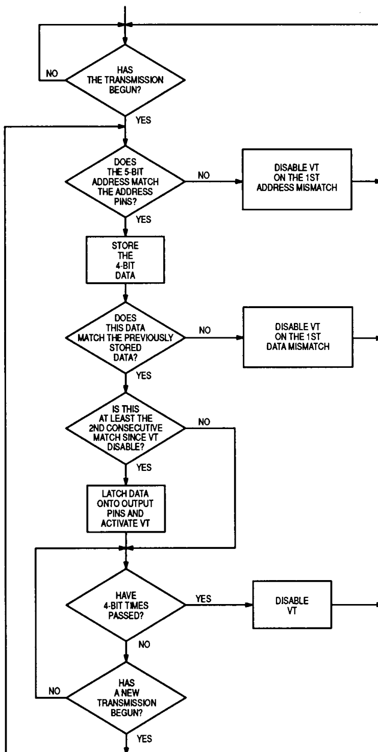
Figure 12. MC145027 Flowchart
