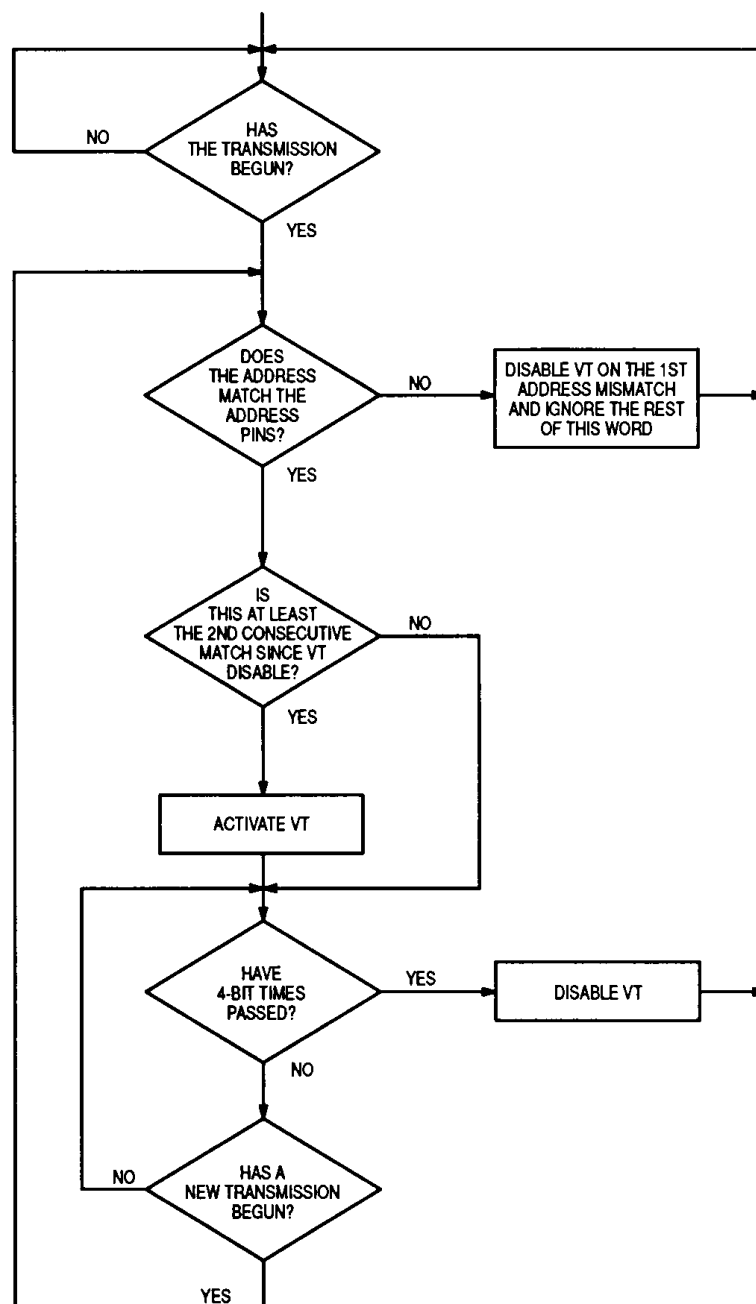
Figure 13. MC145028 Flowchart
