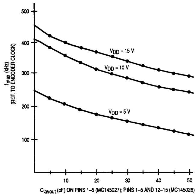
Figure 14. f_{\text{max}} vs C_{\text{layout}} — Decoders Only
