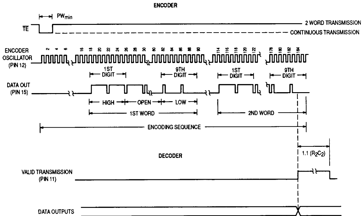
Figure 10. Timing Diagram
