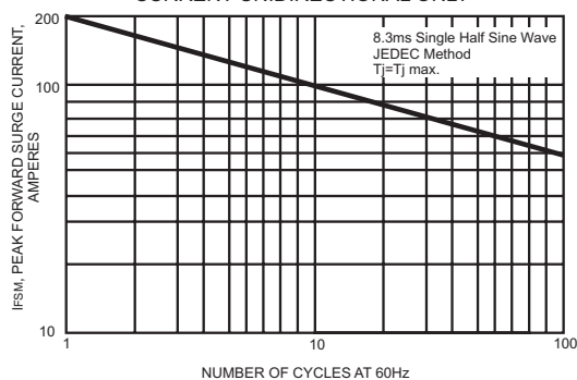
FIG.6- MAXIMUM NON-REPETITIVE FORWARD SURGE CURRENT UNIDIRECTIONAL ONLY
