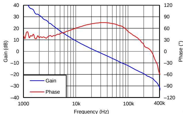
Figure 5. V OUT = 1.8 V, I OUT = 10 A, C OUT1 = 200 µF ceramic, f sw = 500 kHz
