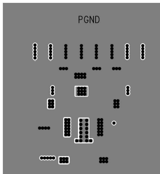
Figure 49. Typical Bottom-Layer Layout
