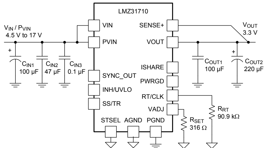
Figure 25. Typical Schematic PVIN = VIN = 4.5 V to 17 V, VOUT = 3.3 V
