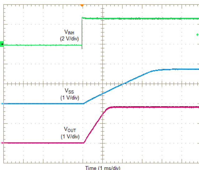
Figure 32. Inhibit Turn-On
