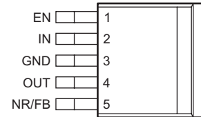
KTT Package 5-Pin TO-263 Top View
