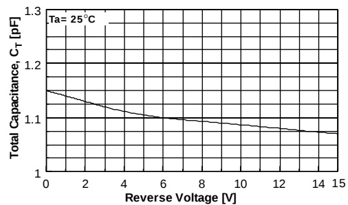
Figure 6. Total Capacitance
