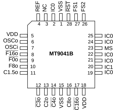
Figure 2 - Pin Connections
