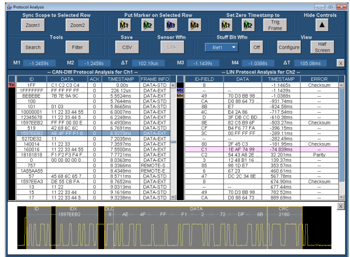
CAN and LIN Timing and Protocol Decode.
