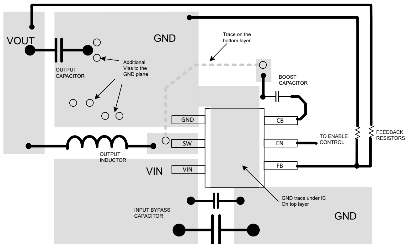
Figure 11-1. Layout
