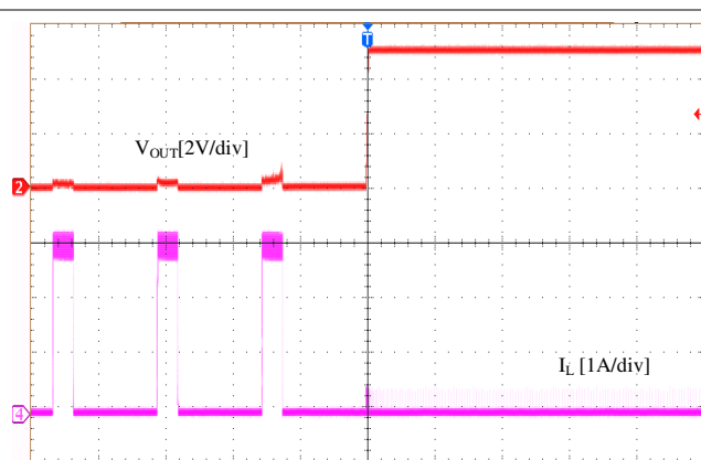
Figure 9-9. Short Recovery
