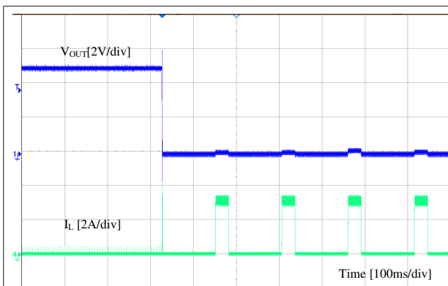
Figure 9-8. Short Protection
