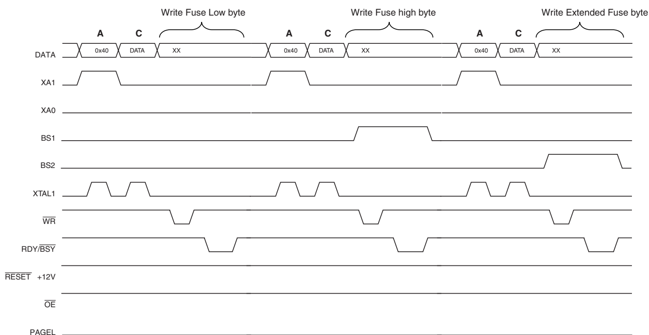
Figure 100. Programming the FUSES Waveforms
