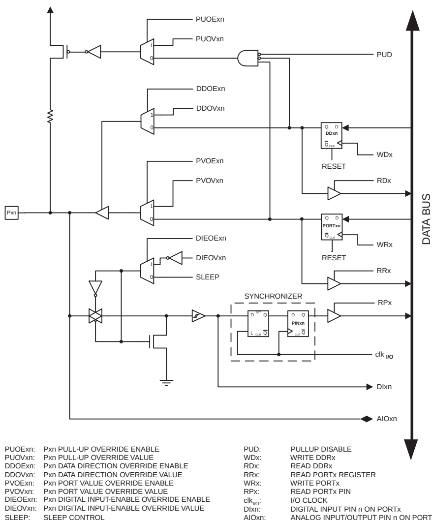
Figure 32. Alternate Port Functions (1)
