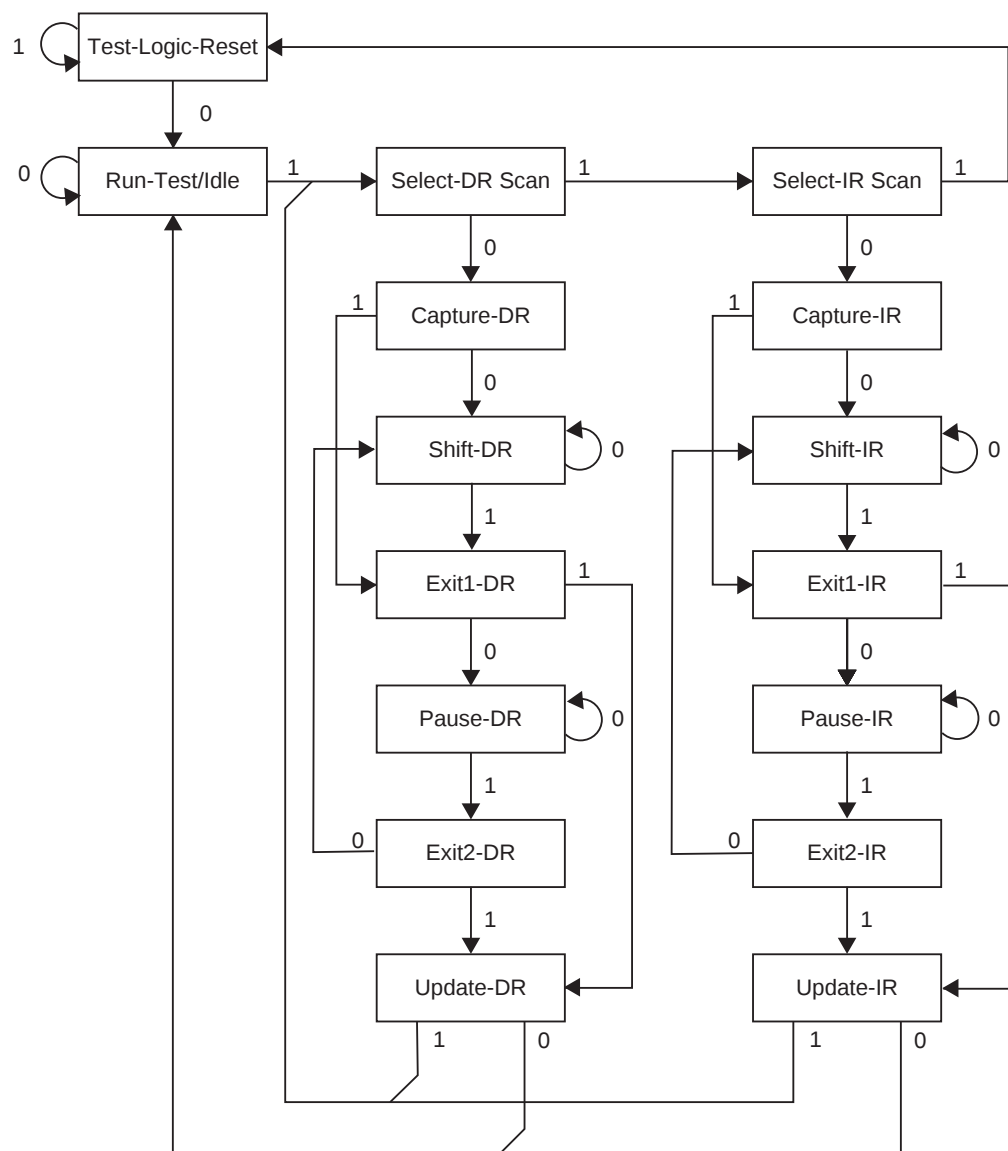
Figure 84. TAP Controller State Diagram
