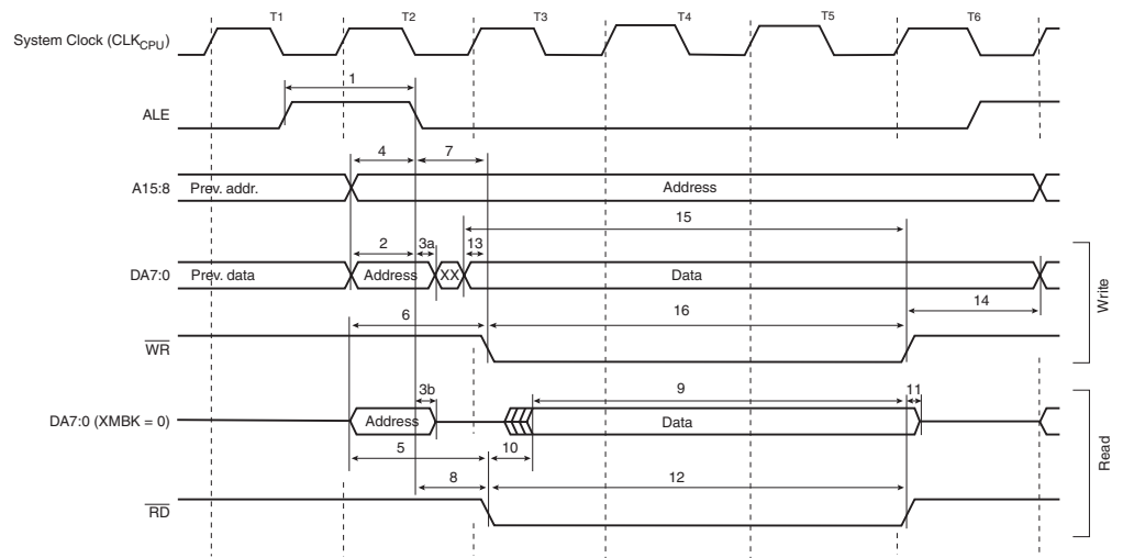
Figure 120. External Memory Timing (SRWn1 = 1, SRWn0 = 0)
