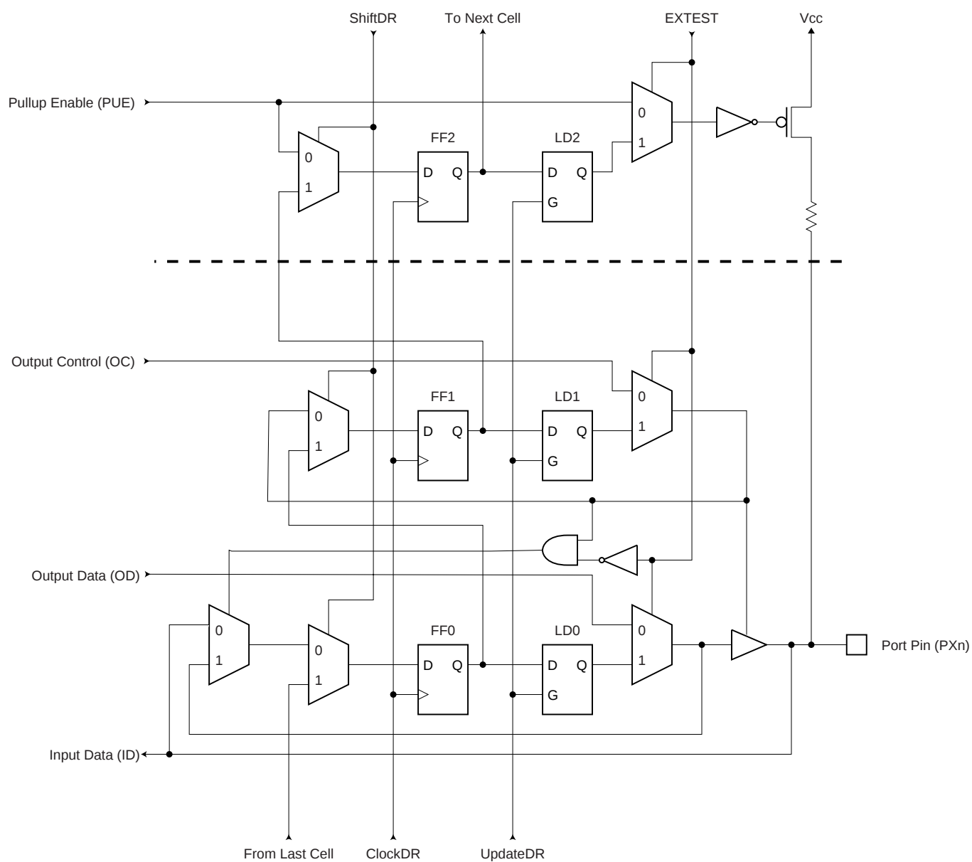
Figure 87. Boundary-scan Cell for Bi-directional Port Pin with Pull-up Function.
