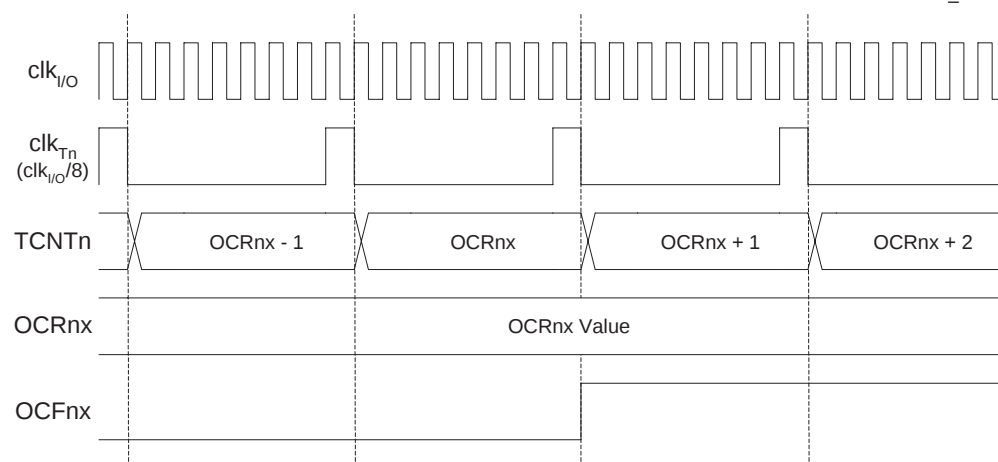
Figure 56. Timer/Counter Timing Diagram, Setting of OCFnx, with Prescaler ( f_{\text{clk\_I/O}}/8 )
