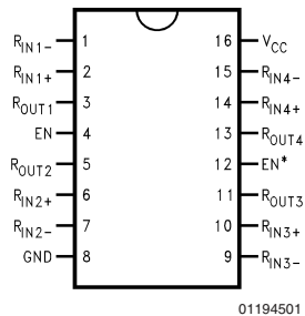
Dual-In-Line
