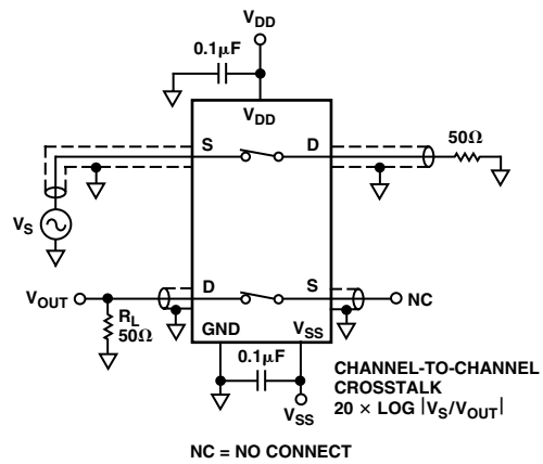
Test Circuit 9. Channel-to-Channel Crosstalk
