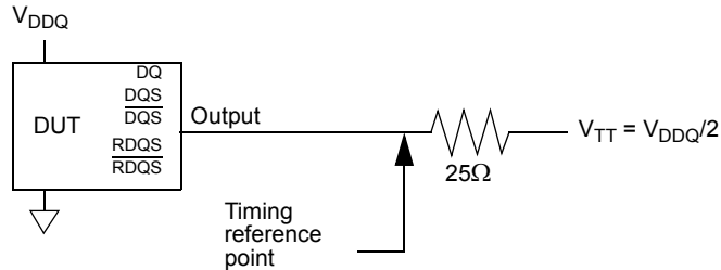
Figure 1 - AC Timing Reference Load
