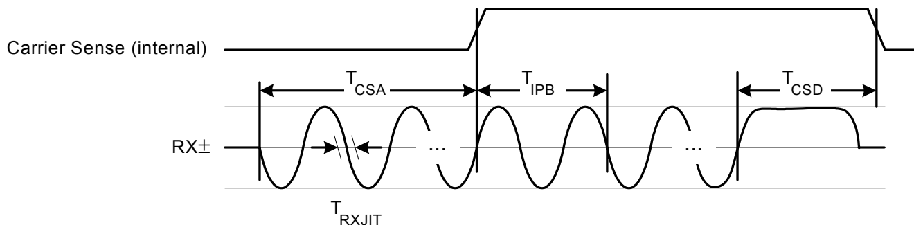
Figure 20. 10BASE-T Receive
