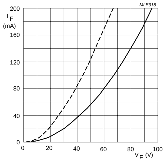
BY8108. Dotted line: T_j = 120\text{ }^{\circ}\text{C} . Solid line: T_j = 25\text{ }^{\circ}\text{C} .
