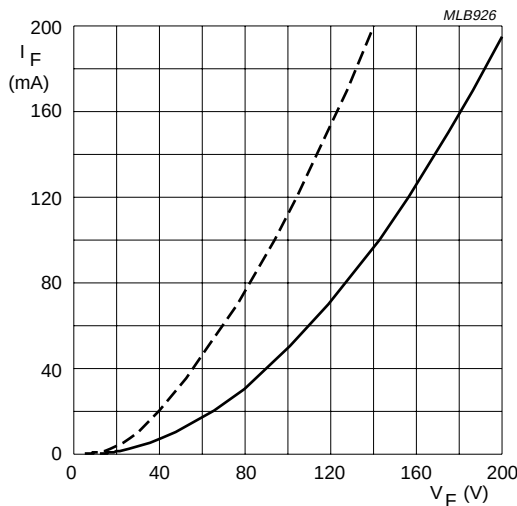
BY8116. Dotted line: T_j = 120\text{ }^{\circ}\text{C} . Solid line: T_j = 25\text{ }^{\circ}\text{C} .
