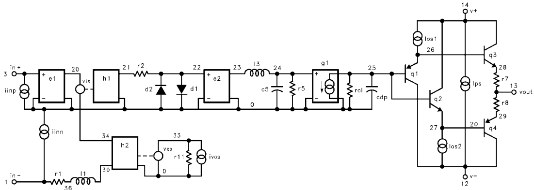
Video Amplifier
