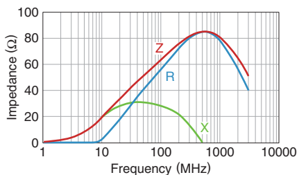
MPZ1608S600A
