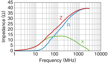
MPZ0603S220C
