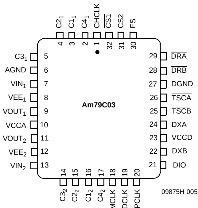
32-Pin PLCC
