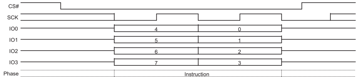
Figure 10.55 Program or Erase Suspend Command Sequence QPI Mode
