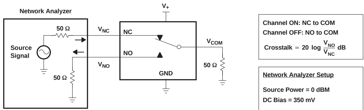
Figure 17. Crosstalk ( X_{\text{TALK}} )
