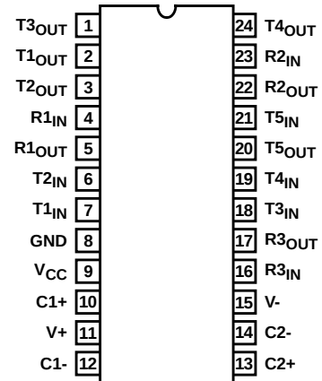
HIN207A (PDIP, SOIC, SSOP) TOP VIEW
