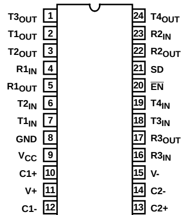
HIN236A (PDIP, SOIC, SSOP) TOP VIEW
