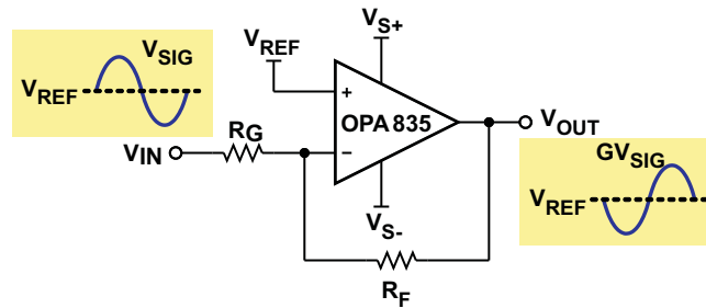
Figure 54. Inverting Amplifier
