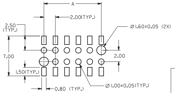
RECOMMENDED SOLDER PAD DESIGN
