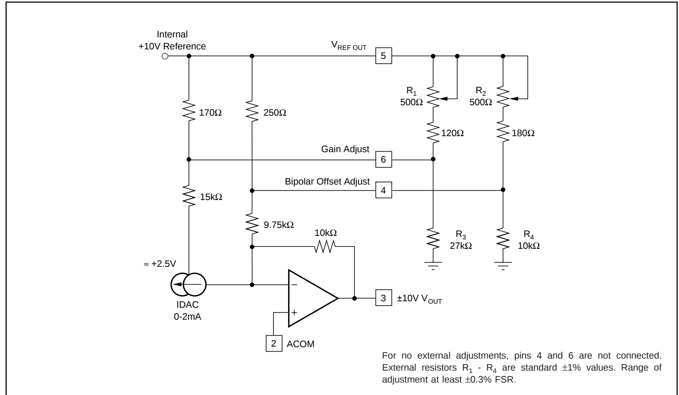
FIGURE 6. Manual Offset and Gain Adjust Circuits.
